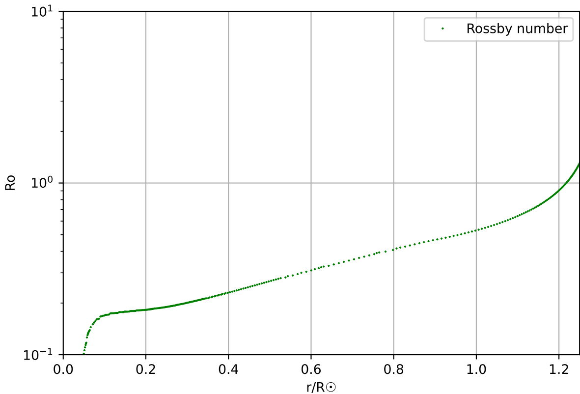
Rossby number, profile 169, age 9.88 \times 10^9
